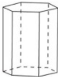
hexagonal prism
