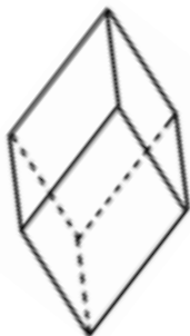
monoclinic prism
